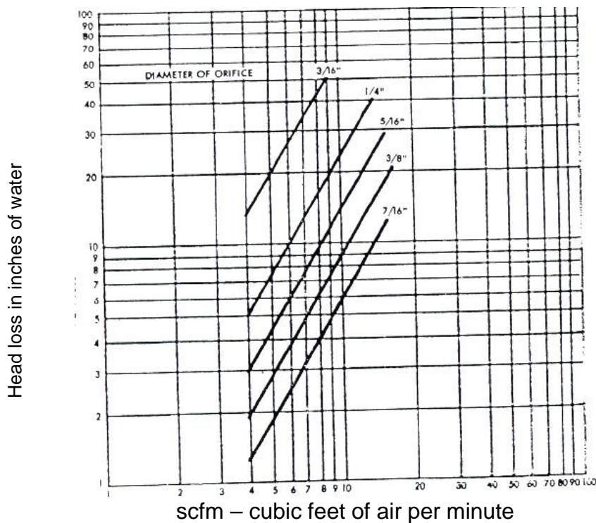
HEAD LOSS CURVE SA-P AIR COMB 3/4" ABS NIPPLE WITH 2 ORIFICES
